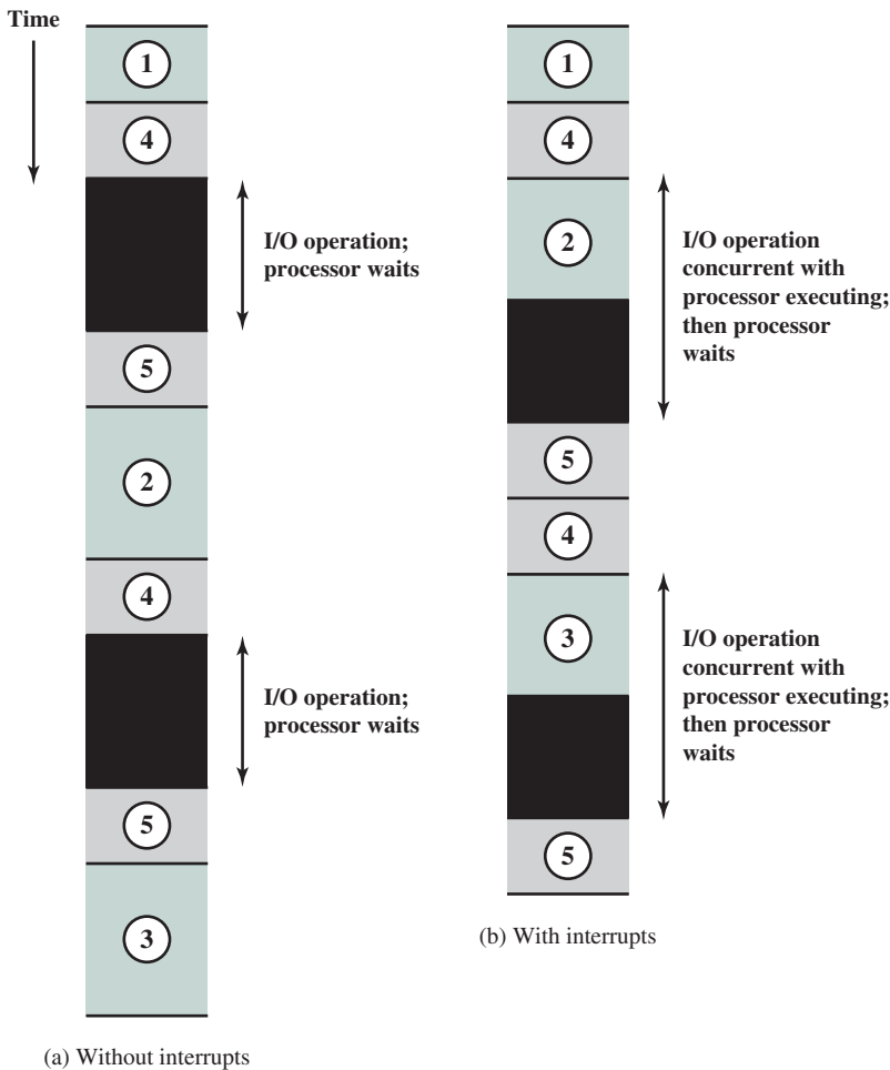
Figure 3.11 Program Timing: Long I/O Wait
