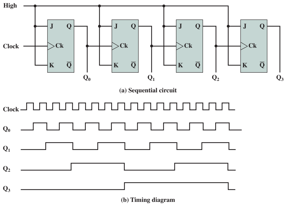
Figure 11.30 Ripple Counter
