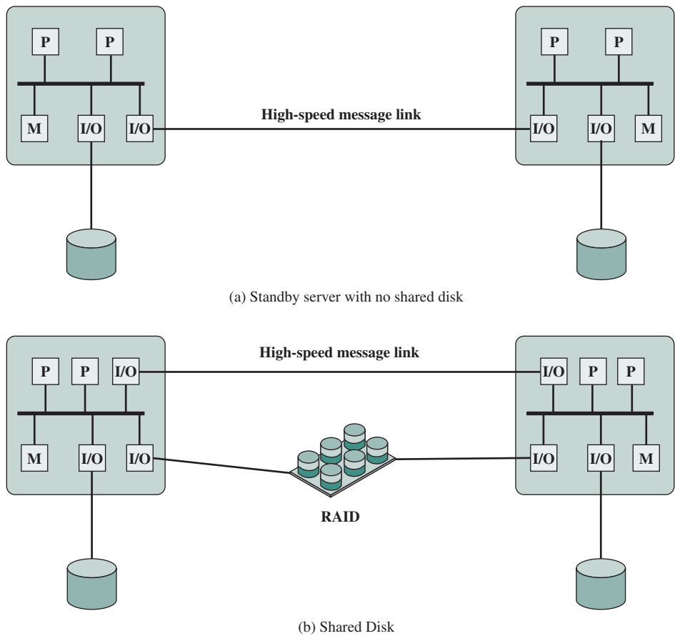
Figure 17.8 Cluster Configurations
