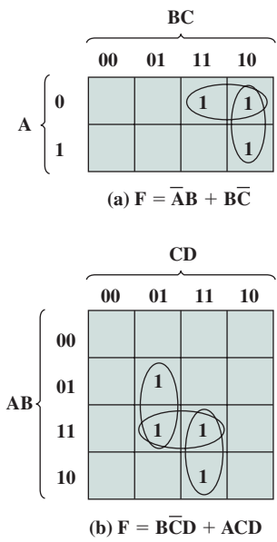
Figure 11.9 Overlapping Groups
