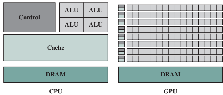
Figure 19.2 CPU versus GPU Silicon Area/Transistor Dedication
