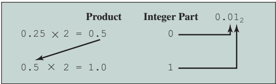
(b) 0.25_{10} = 0.01_2 (exactly)
