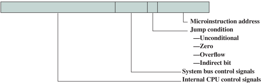
(a) Horizontal microinstruction
