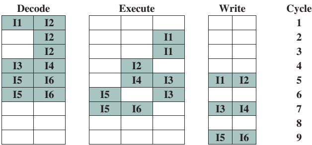
Figure 16.14 An In-Order Issue, In-Order-Completion Execution Sequence
