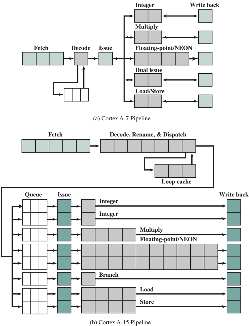
Figure 18.10 Cortex A-7 and A-15 Pipelines
