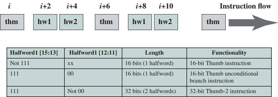
Figure 13.13 Thumb-2 Encoding
