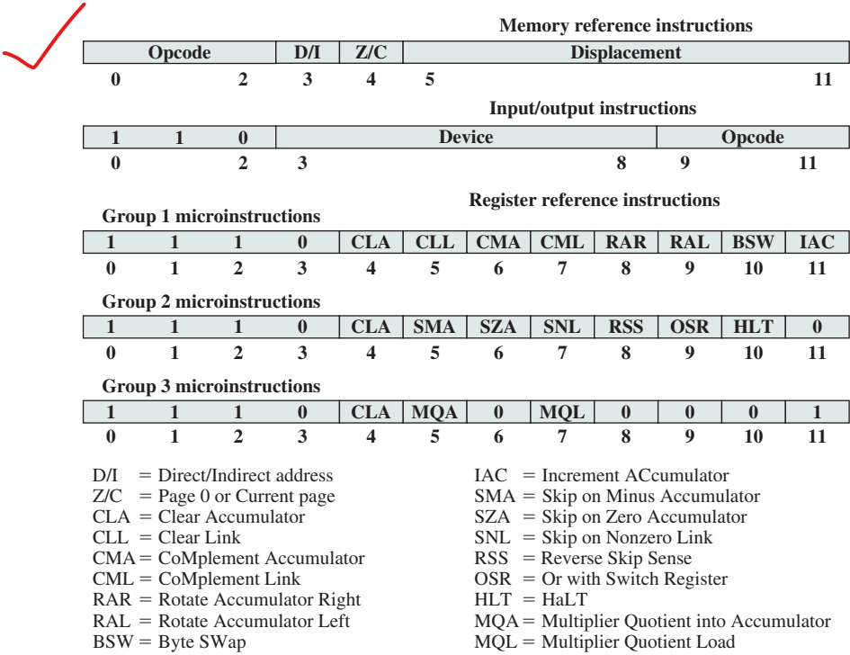
Figure 13.5 PDP-8 Instruction Formats
