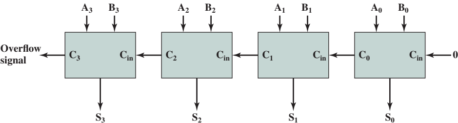
Figure 11.19 4-Bit Adder
