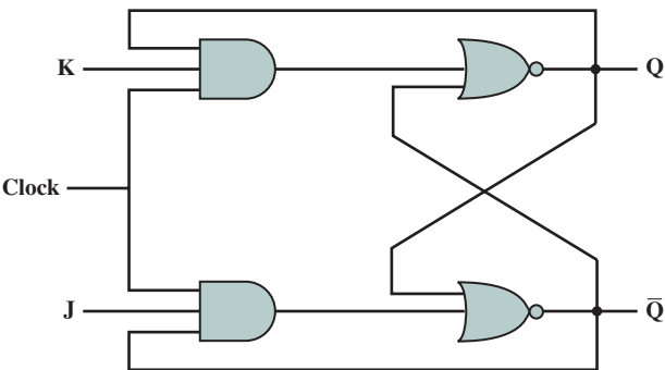
Figure 11.26 J-K Flip-Flop
