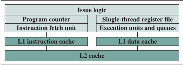
(a) Superscalar
