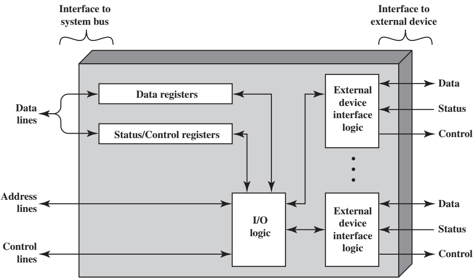
Figure 7.3 Block Diagram of an I/O Module
