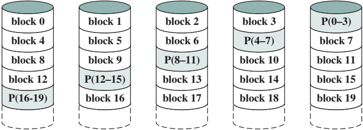
(f) RAID 5 (Block-level distributed parity)
