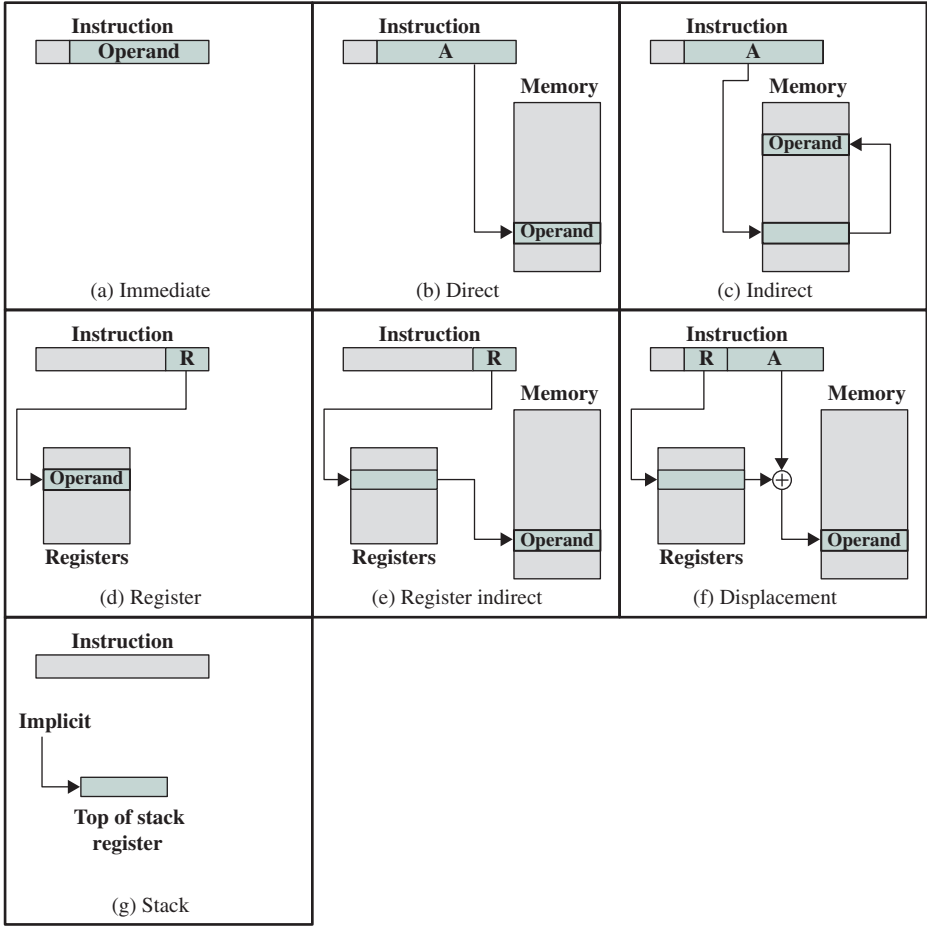
Figure 13.1 Addressing Modes
