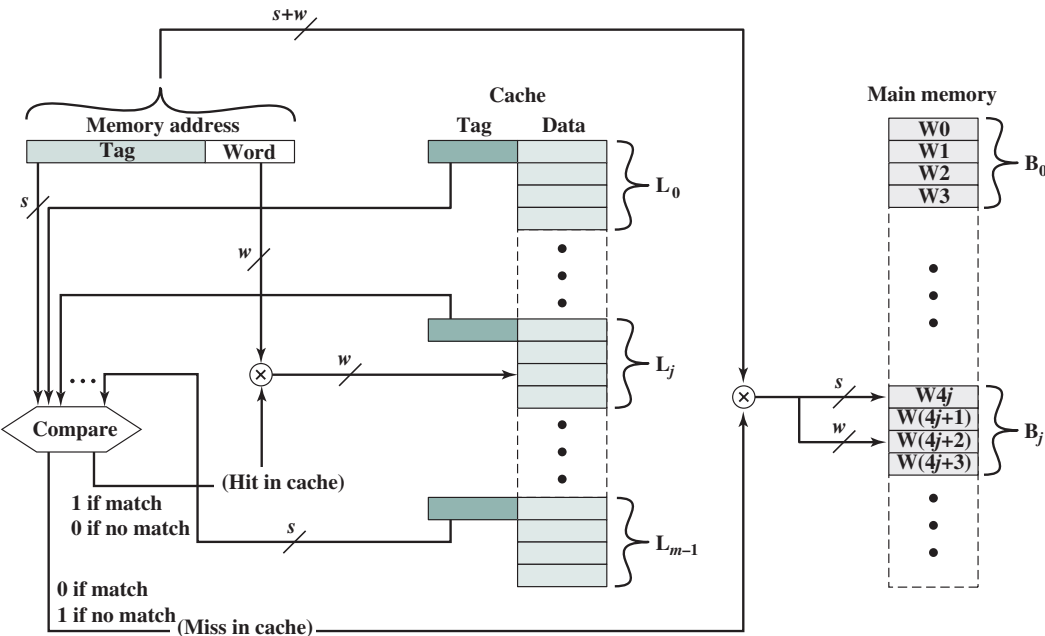
Figure 4.11 Fully Associative Cache Organization
