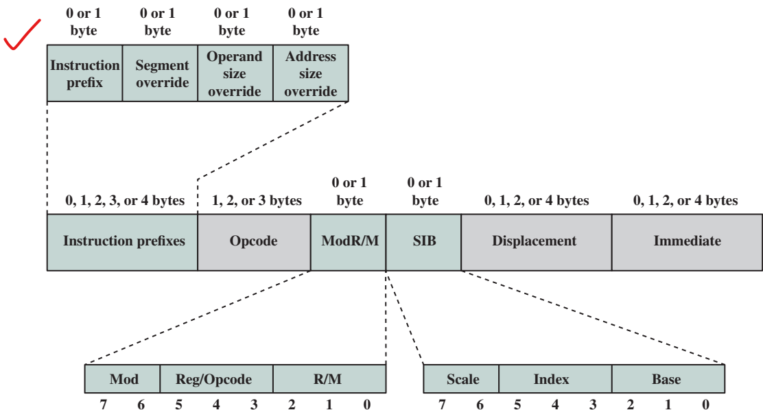
Figure 13.9 x86 Instruction Format
