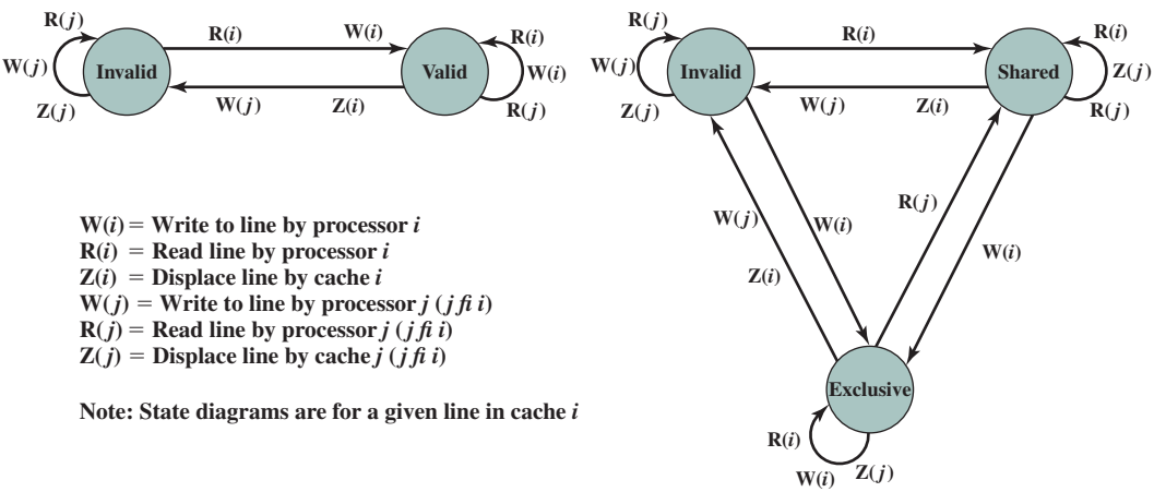
Figure 17.17 Two Cache Coherence Protocols
