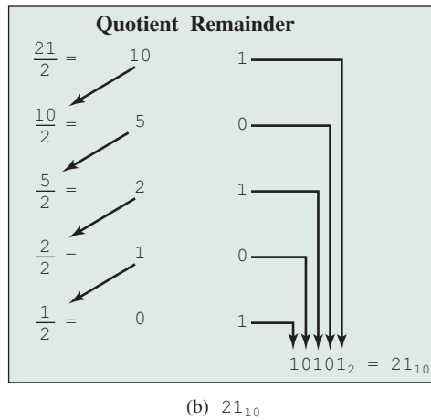
Figure 9.1 Examples of Converting from Decimal Notation to Binary Notation for Integers
