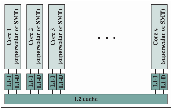
(c) Multicore
