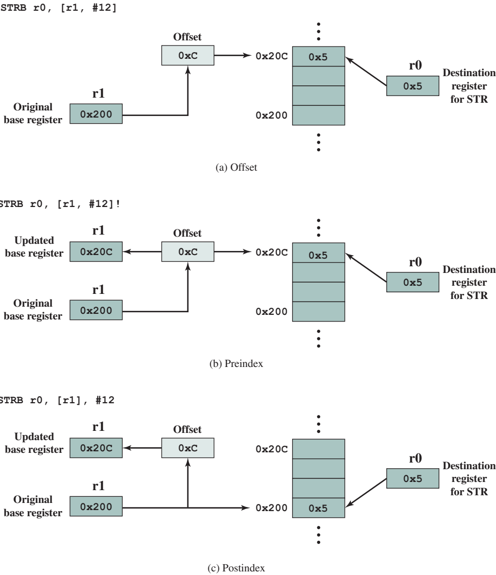
Figure 13.3 ARM Indexing Methods
