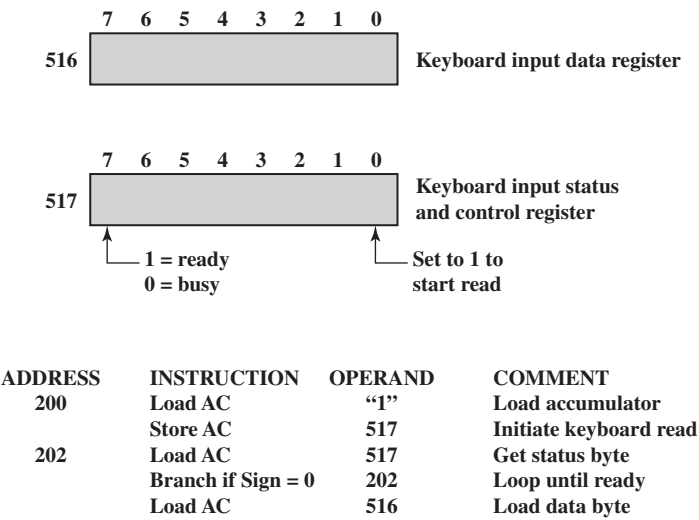
(a) Memory-mapped I/O
